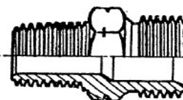
NIPPLIO RIDOTTO GAS CILINDRICO SVASATO X NPT REDUCED NIPPLE BSP FLARED X NPT
