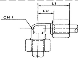
RACCORDO INTERMEDIO A GOMITO SERIE LL (DIN 2353) INTERMEDIATE FITTING ELBOW SERIES LL (DIN 2353)
