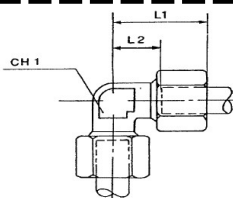
RACCORDO INTERMEDIO A GOMITO SERIE L (DIN 2353) INTERMEDIATE FITTING ELBOW SERIES L (DIN 2353)
