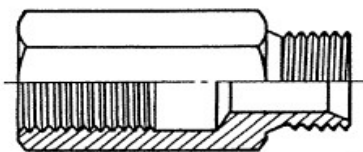
PROLUNGA MASCHIO GAS CILINDRICO SVASATO X FEMMINA FISSA GAS EXTENSION BSP MALE FLARED X FIXED BSP FEMALE
