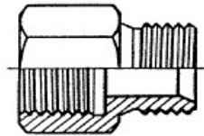
PROLUNGA CORTA MASCHIO GAS CILINDRICO SVASATO X FEMMINA FISSA GAS SHORT EXTENSION BSP MALE FLARED X FIXED BSP FEMALE
