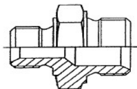
NIPPLE RIDOTTO GAS CILINDRICO SVASATO X GAS CILINDRICO SVASATO REDUCED NIPPLE BSP FLARED X BSP FLARED
