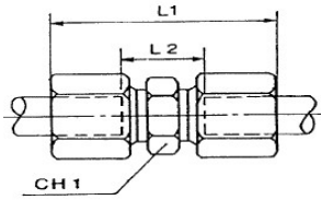
RACCORDO INTERMEDIO DIRITTO SERIE LL (DIN 2353) INTERMEDIATE FITTING STRAIGHT SERIES LL (DIN 2353)
