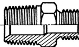
NIPPLIO RIDOTTO GAS CILINDRICO SVASATO X GAS CONICO REDUCED NIPPLE BSP FLARED X BSP TAPERED
