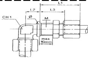
RACCORDO PASSAPARETE A GOMITO SERIE S (DIN 2353) BULKHEAD ELBOW FITTING SERIES S (DIN 2353)
