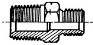
NIPPLIO RIDOTTO GAS CILINDRICO SVASATO X NPT REDUCED NIPPLE BSP FLARED X NPT
