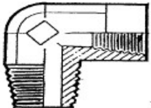
GOMITO FEMMINA FISSA X GAS CONICO MASCHIO ELBOW FIXED FEMALE X BSP TAPERED MALE
