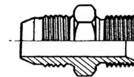
NIPPLIO GAS CILINDRICO SVASATO X JIC-UNF-NF NIPPLE BSP FLARED X JIC-UNF-NF
