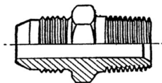
NIPPLO GAS CONICO X JIC-UNF-NF NIPPLE BSP TAPERED X JIC-UNF-NF
