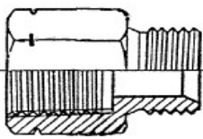
PROLUNGA CORTA MASCHIO GAS CILINDRICO SVASATO X FEMMINA FISSA NPT SHORT EXTENSION BSP MALE FLARED X FIXED NPT FEMALE
