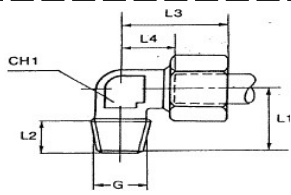
RACCORDO DI ESTREMITA' A GOMITO GAS - CONICO SERIE LL (DIN 2353) EXTREMITY ELBOW FITTING BSP TAPERED SERIES LL (DIN 2353)
